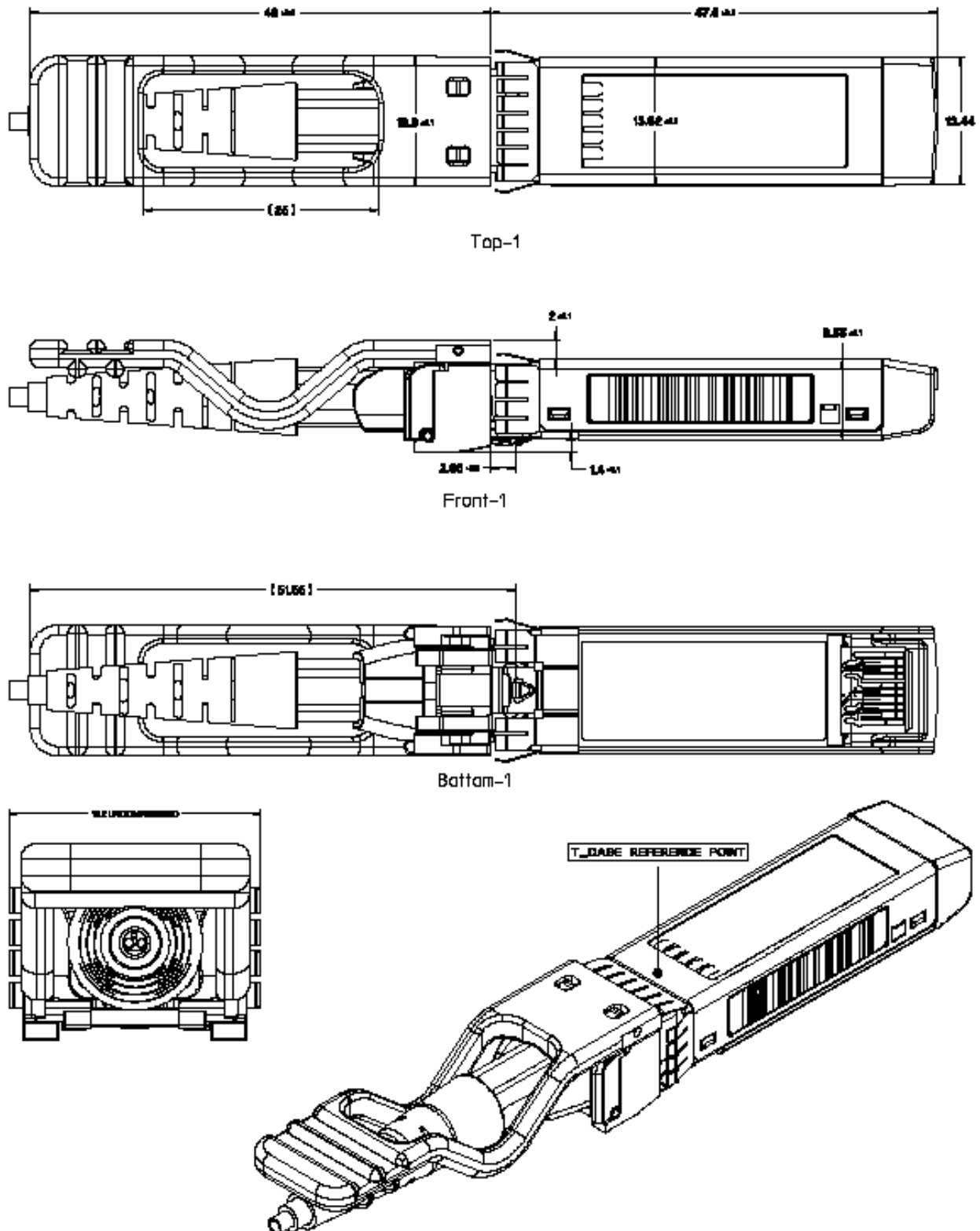
Figure 4. Module drawing
