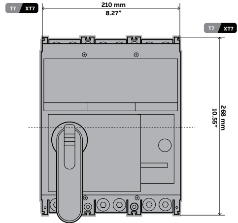
T7/XT7 FRAME SIZE FRONT COMPARISON
