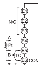
Temperature Indicator K3HB-H
