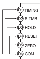
Models with Terminal Blocks <K35-1><K35-3>
