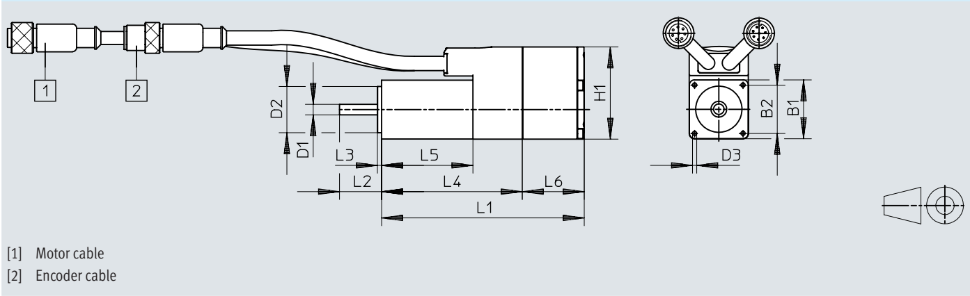
Dimensions – Stepper motors EMMS-ST-...-SB/SEB, size 28 Download CAD data → www.festo.com
