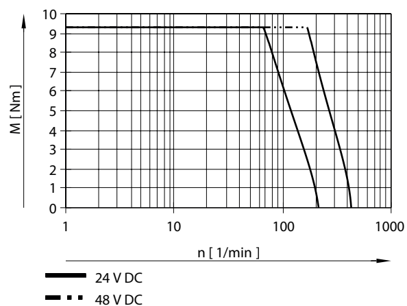
Torque M as a function of rotational speed n for EMMS-ST-87, long
