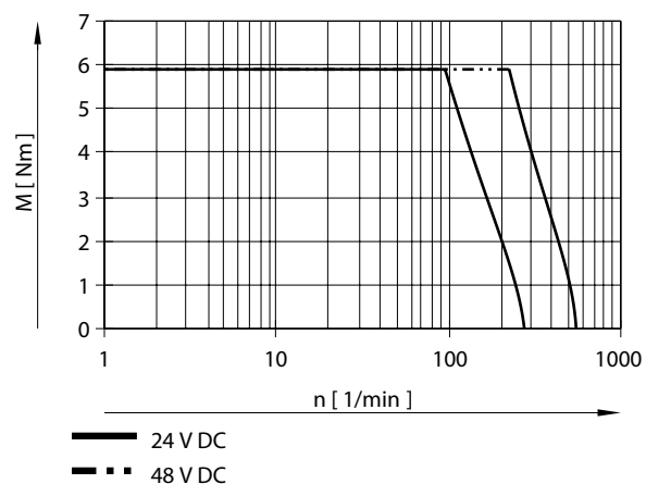
Torque M as a function of rotational speed n for EMMS-ST-87, medium
