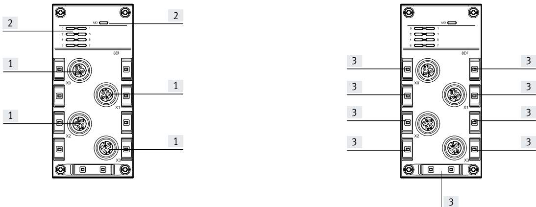
[1] Electrical connection, inputs [2] LED indicators [3] Space for inscription label
